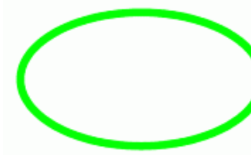
ellipse
