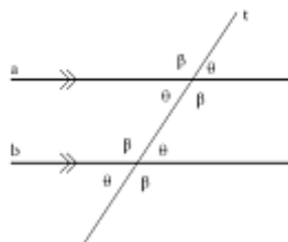
parallel
