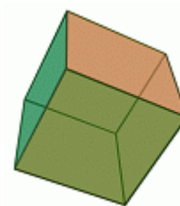
block
