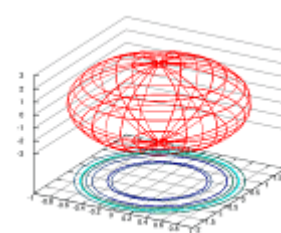
ellipsoid
